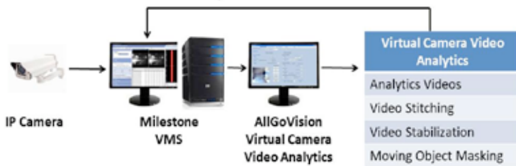
AllGoVision Virtual Camera Video Analytics
